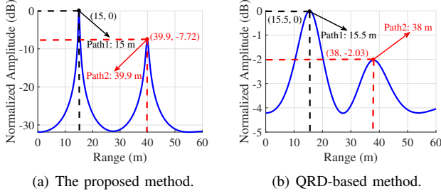
Fig. 8. Performance comparison on distance estimation when the two paths differ significantly.
