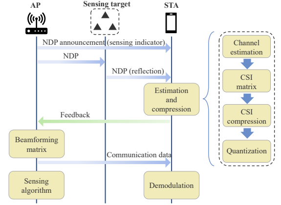
Fig. 2. The proposed ISAC-oriented channel sounding protocol.
